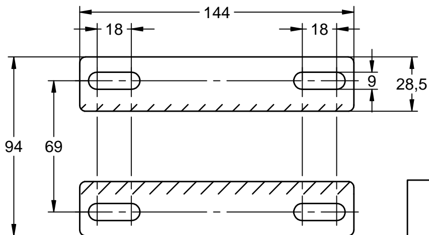
Fastening Plate A-A
