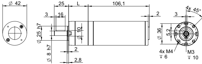
DRAWING (mm)
