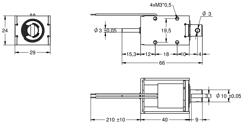
DRAWING (mm)
